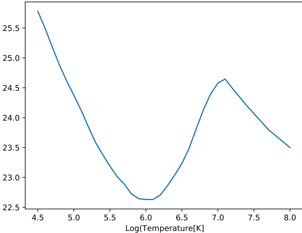
Differential emission measure of the (non-flaring) quiet sun
