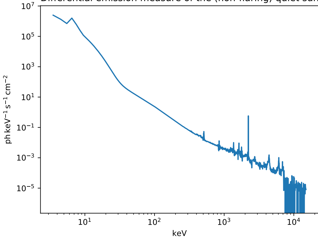
Differential emission measure of the (non-flaring) quiet sun
